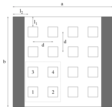
Fig. 3 Different array parameters and element numbering
