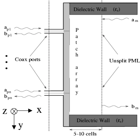
Fig. 2 The analyzed structure (top view).
