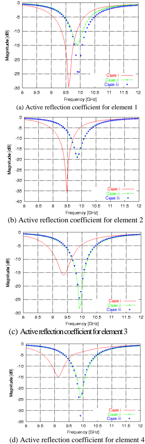
Fig. 5 Active reflection coefficients for different elements
