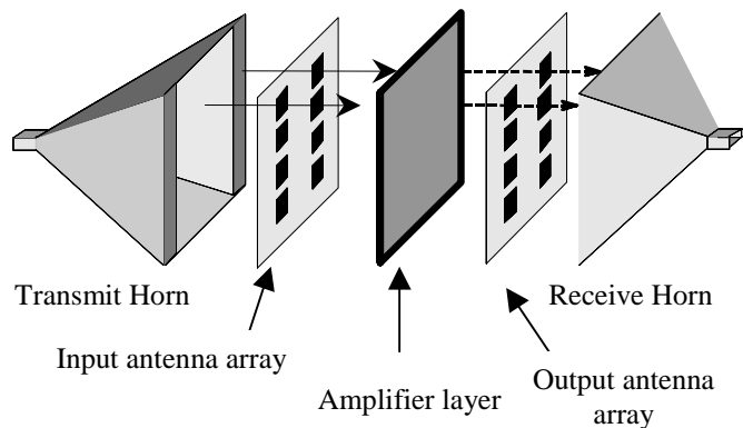
Fig. 1 A general waveguide-based spatial power combining system.
