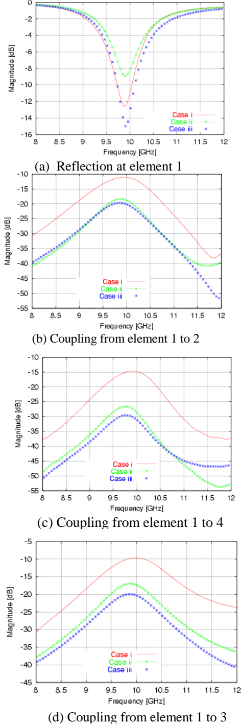
Fig. 4 Reflection and coupling coefficients at element 1
